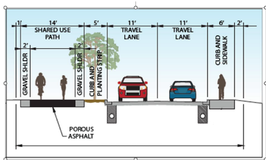
TYPICAL ROADWAY SECTION
