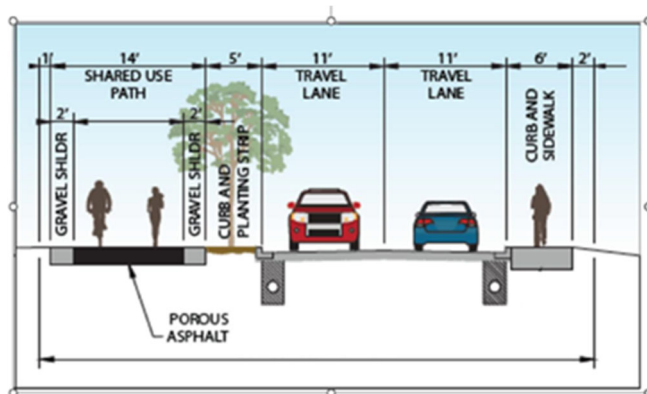
TYPICAL ROADWAY SECTION
